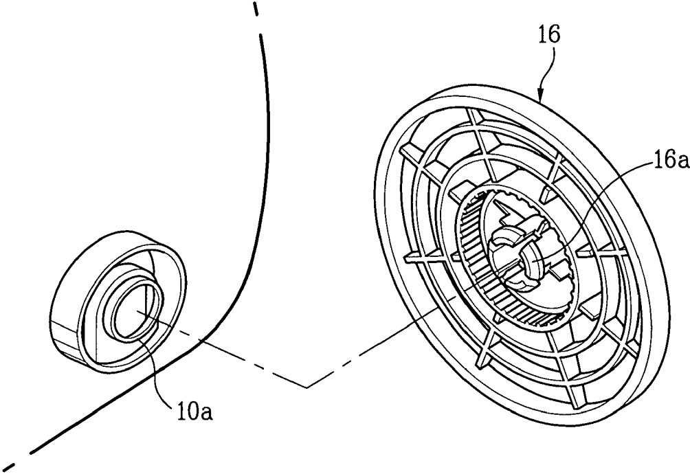
FIG. 3 Prior Art
